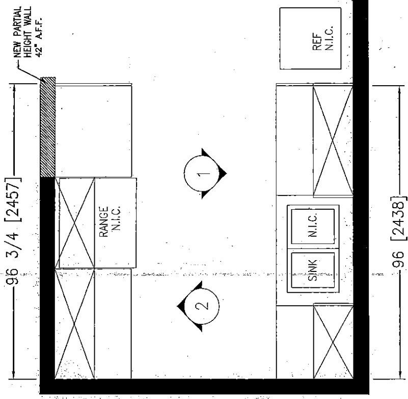
PLAN VIEW
