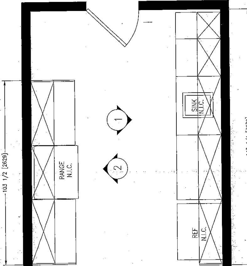
PLAN VIEW
